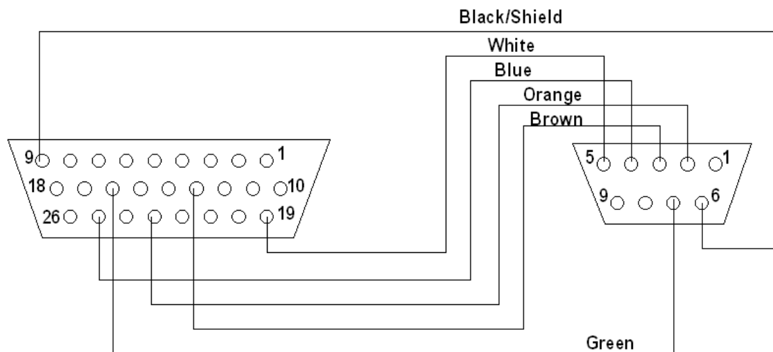
BDR-1500/4500 (Back View)
